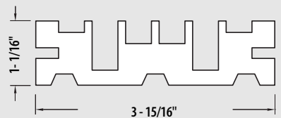
FlutterFree® End View
